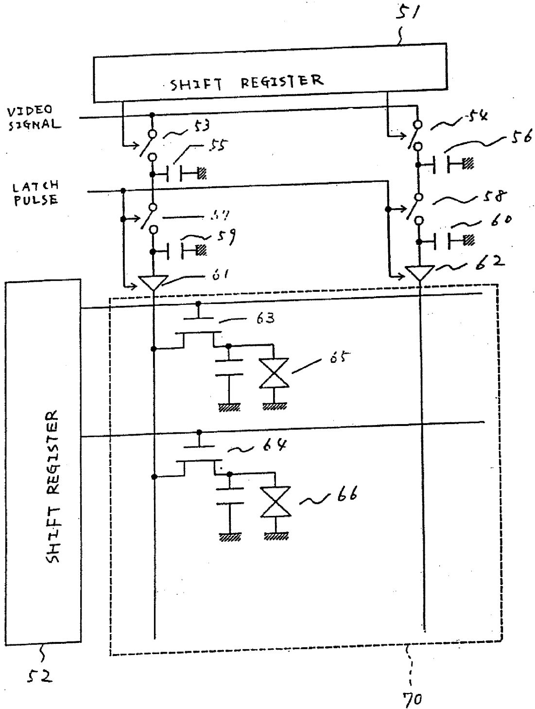
FIG. 5 PRIOR ART
