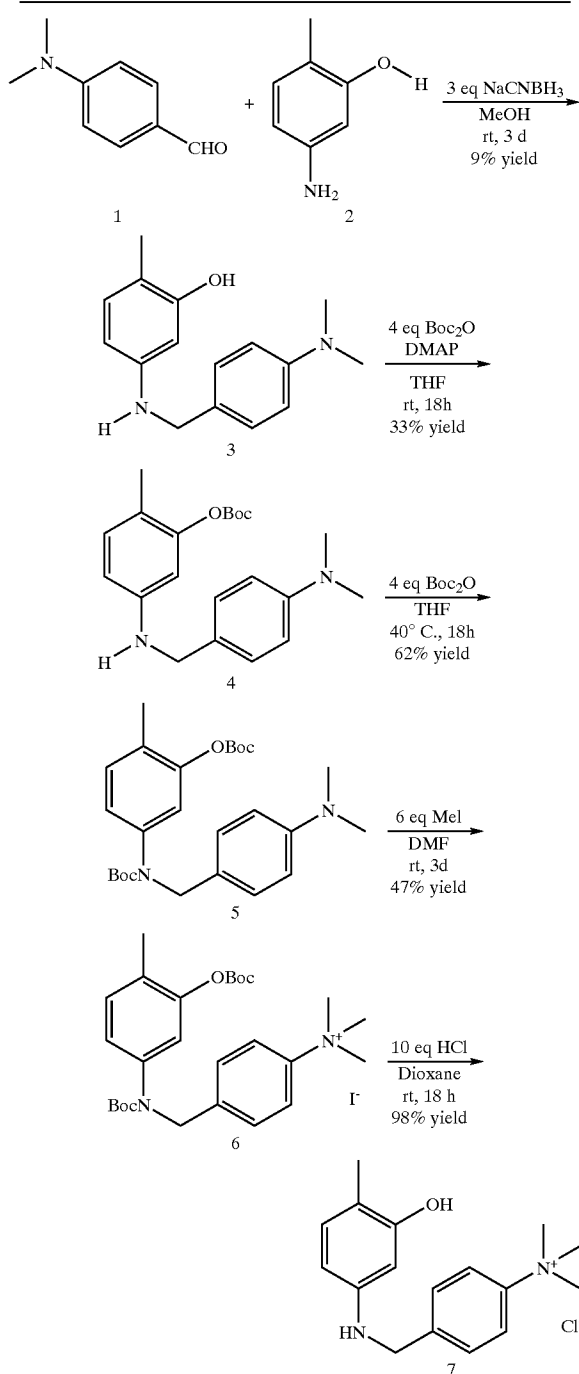
Scheme 1. Synthesis of {4-[3-hydroxy-4-methyl-phenylamino)-methyl]-phenyl}-trimethyl-ammonium chloride 7
