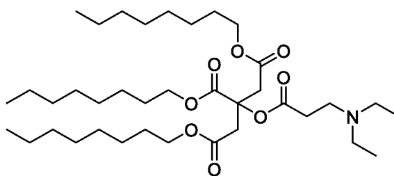
Compound (2)
