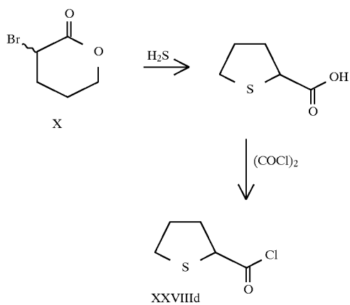
Scheme 6
