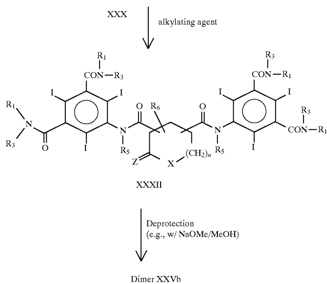
Scheme 3
