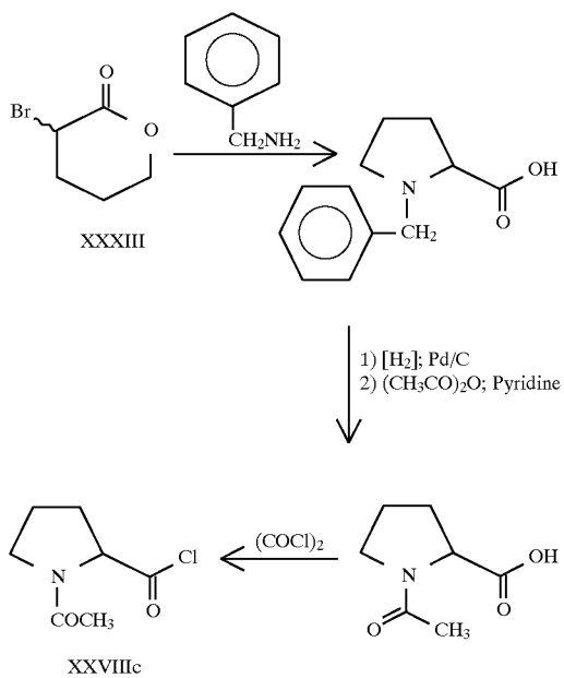
Scheme 5
