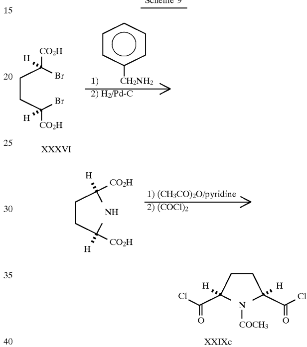
Scheme 9
