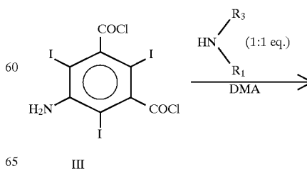
Scheme 11
