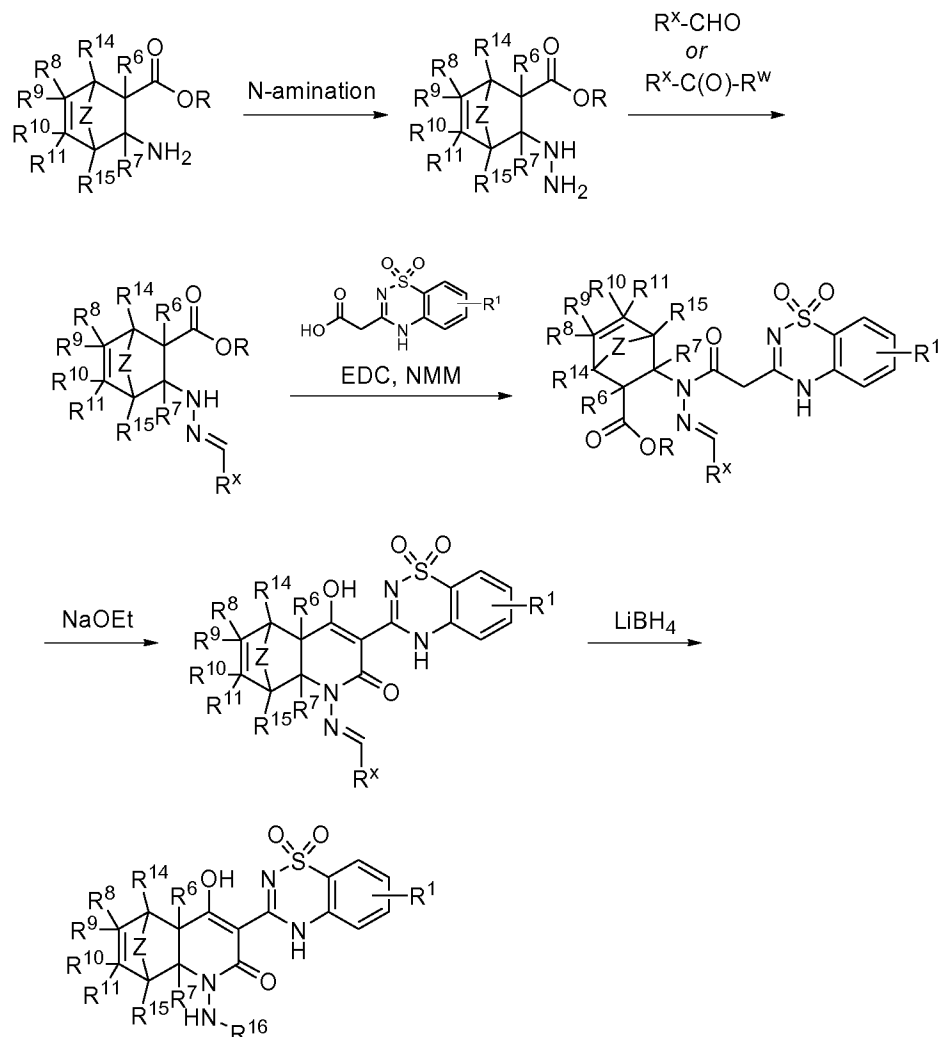
Scheme 36
