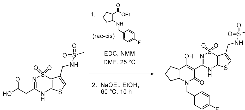
Scheme 29
