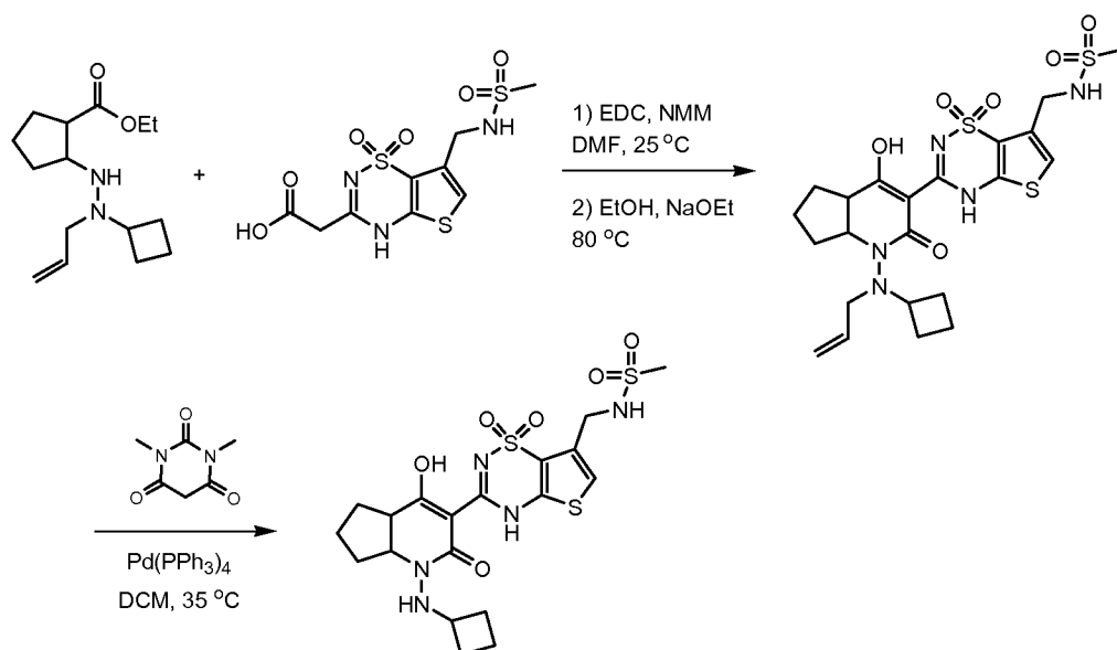
Scheme 37
