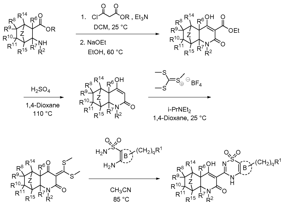
Scheme 25
