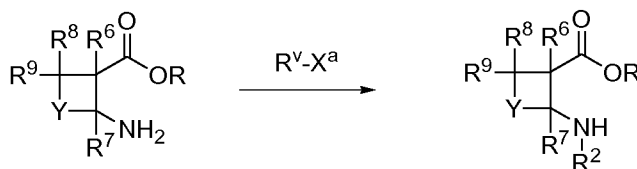
Scheme 15
