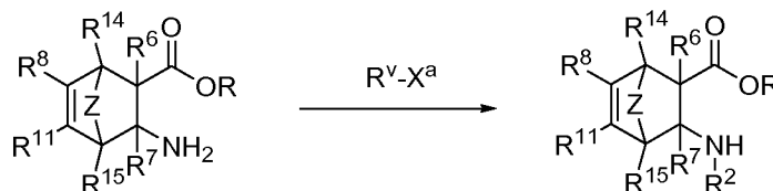
Scheme 12
