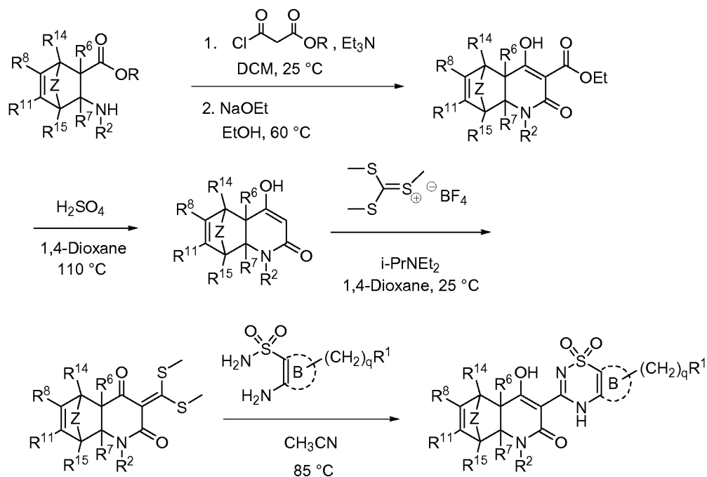
Scheme 27
