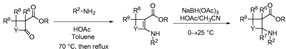
Scheme 16
