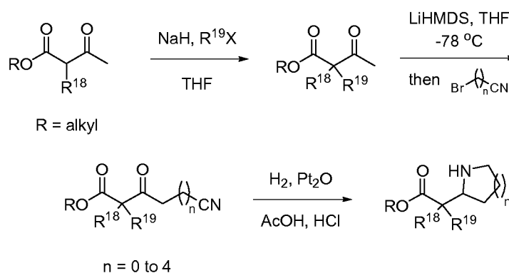
Scheme 23
