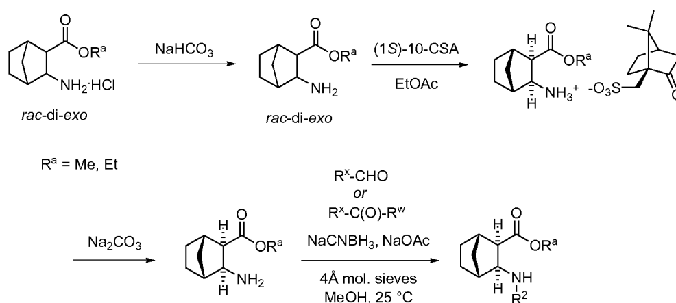
Scheme 5
