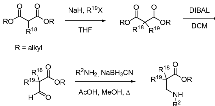
Scheme 20
