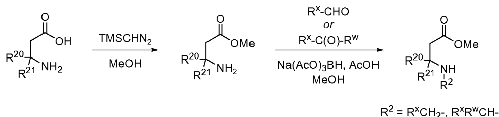
Scheme 22
