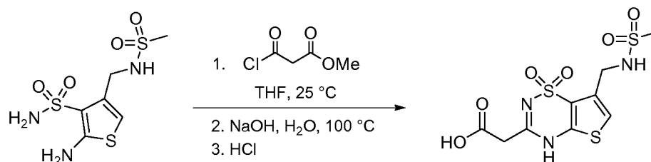
Scheme 32
