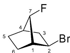
2- exo -bromo-7- syn -fluoro-bicyclo[2.2.1]heptane
