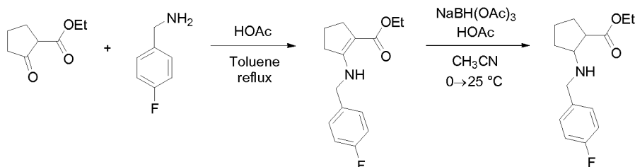
Scheme 17
