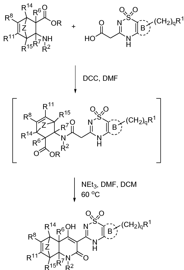
Scheme 9
