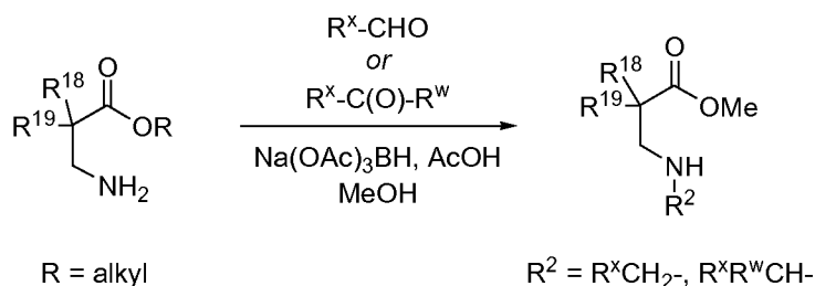
Scheme 21
