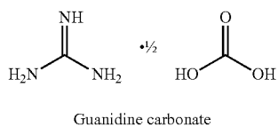
Guanidine carbonate
