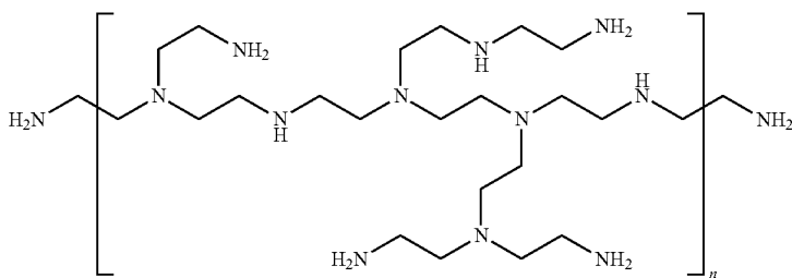
Branched Polyethylenimine
