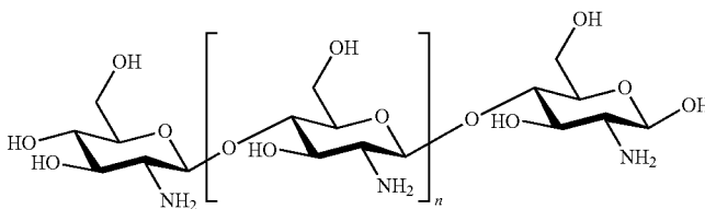
Chitosan
