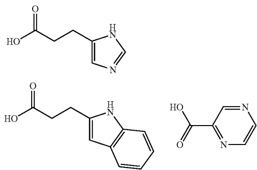
Chart 1: Representative acids for amination reactions.
