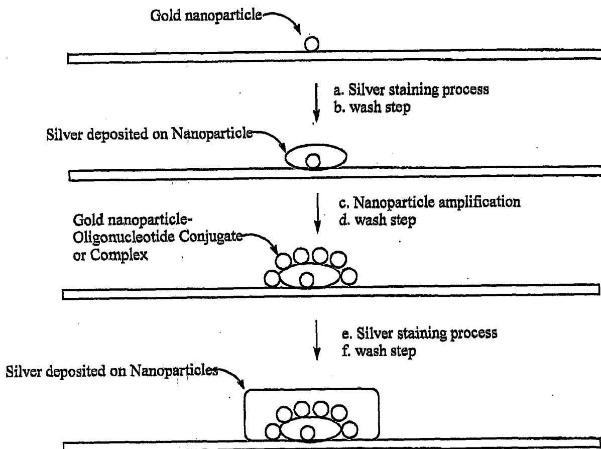
Figure 1. Schematic representation of amplification of a detection signal for a gold nanoparticle immobilized on a solid surface. Step "a" is conventional silver staining. In step "c" gold nanoparticles bearing oligonucleotides are bound to the silver surface. Step "e" is conventional silver staining of the gold nanoparticles that were bound to the previous silver surface.
