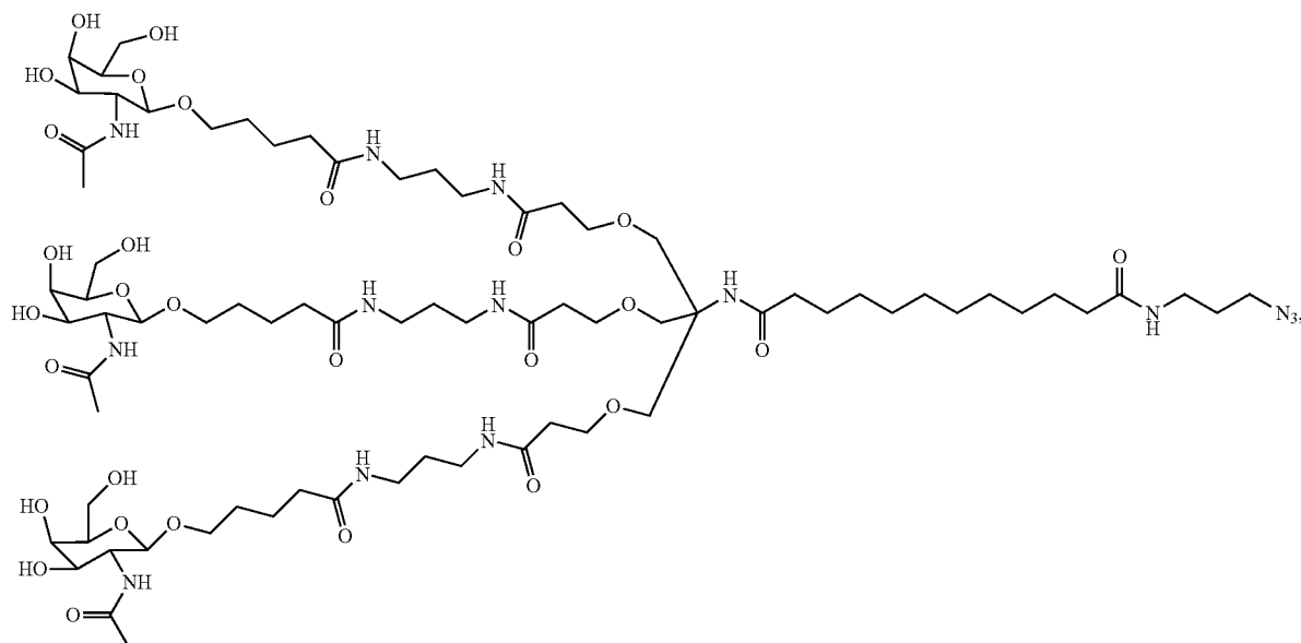
(Molecule I')
