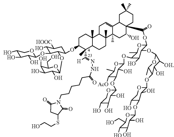
(Molecule 3)
