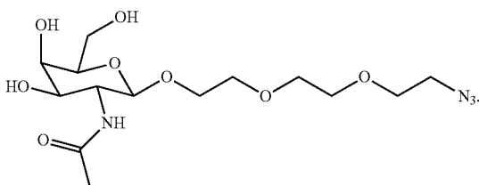
(Molecule II')
