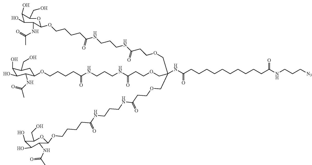
(Molecule I')
