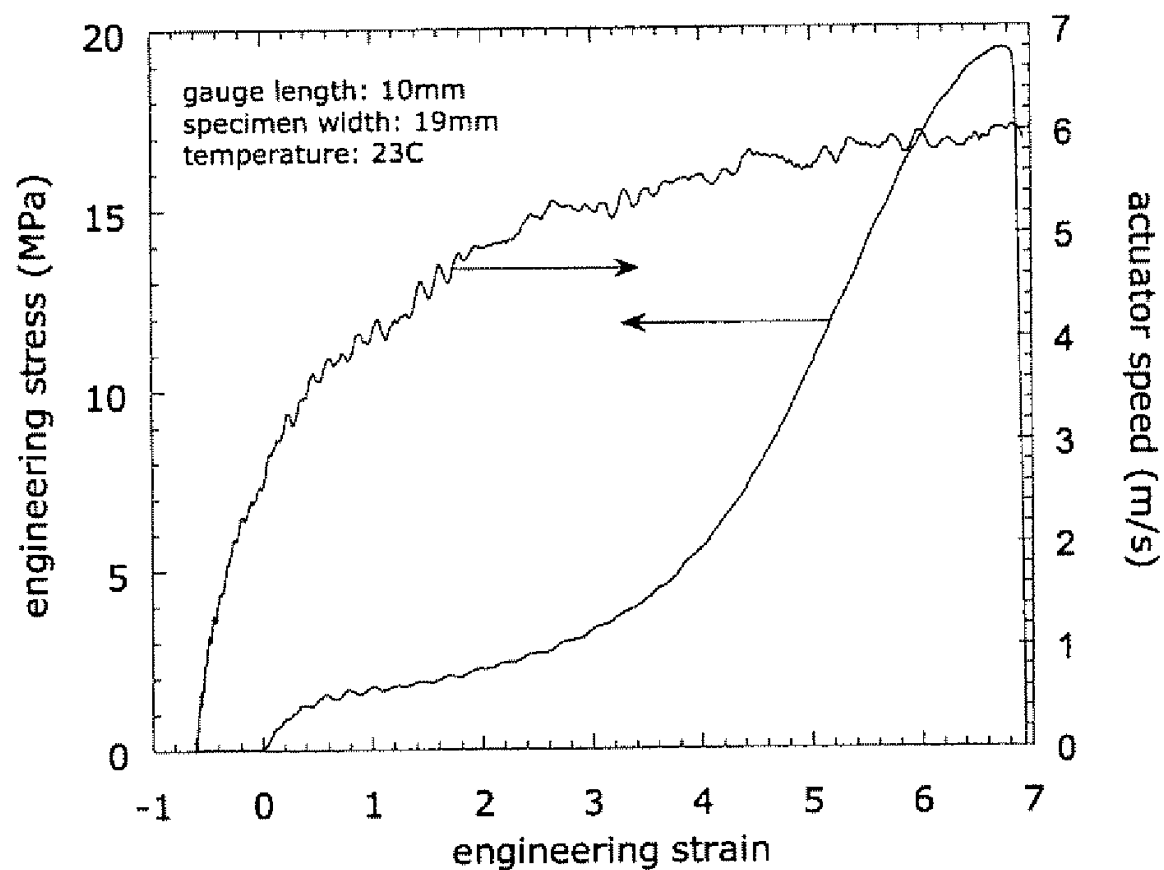
Stress and Actuator Speed During High Speed Tensile Test
