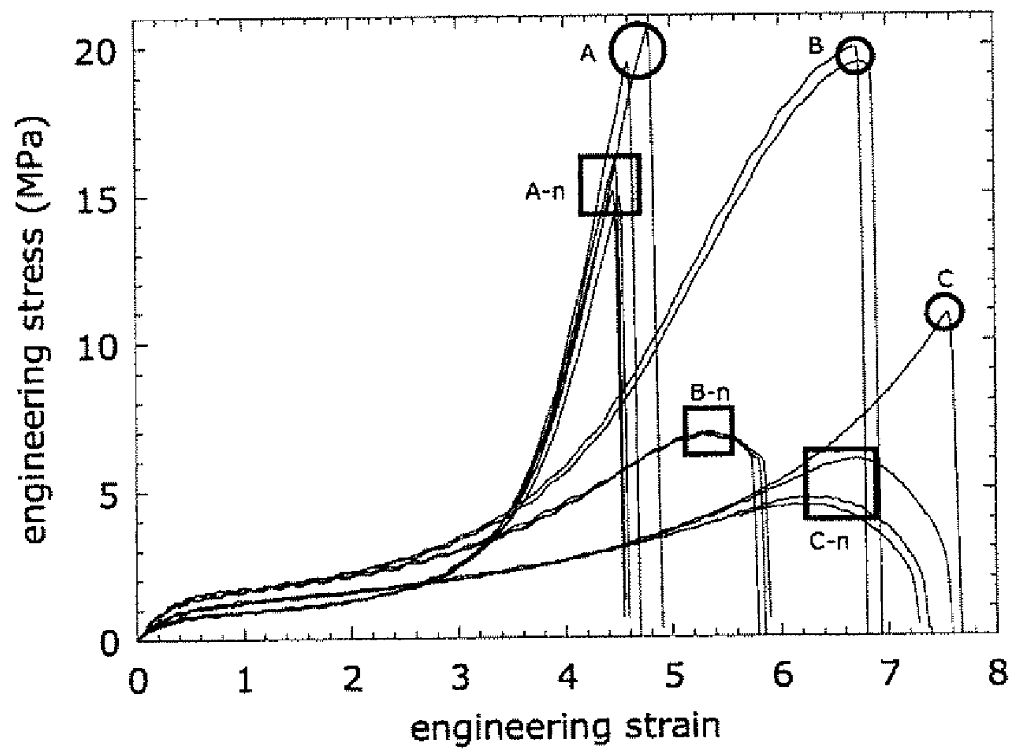
High Speed Tensile Results: Three Films
