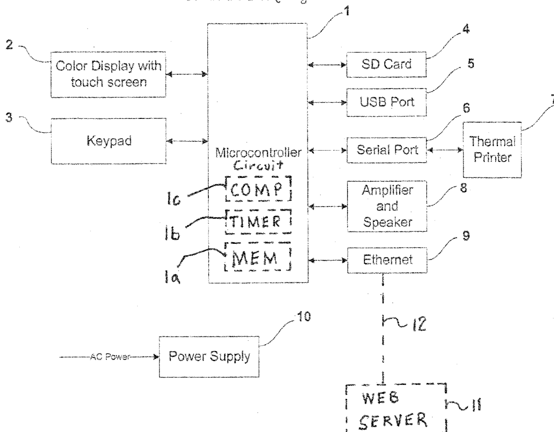
Product Rotation Label System Hardware Block Diagram
