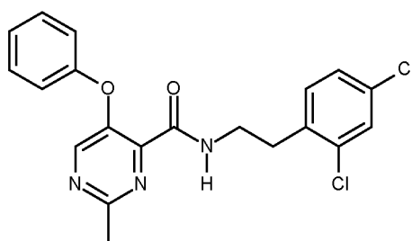
Compound A-1.20
