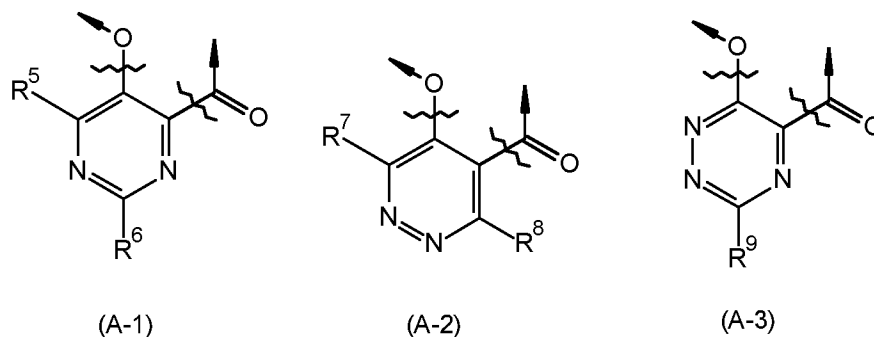
Scheme 7
