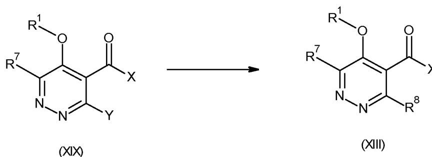
Scheme 14
