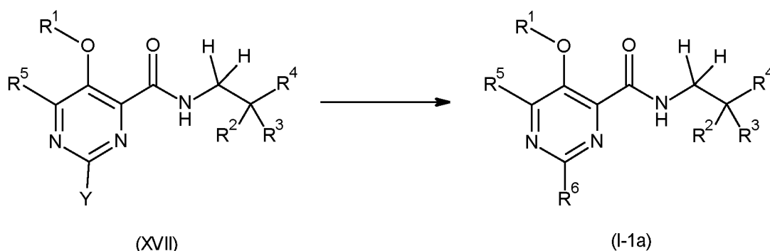
Scheme 11
