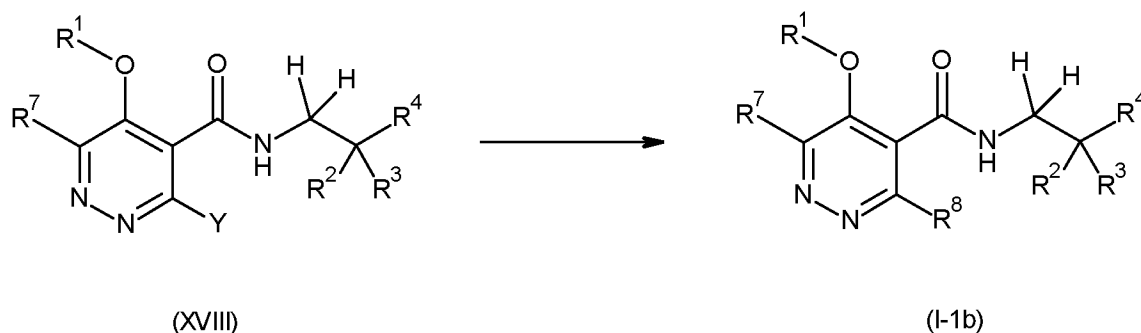
Scheme 12
