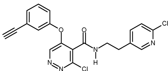
Compound B-10.9
