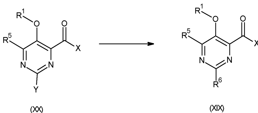
Scheme 13
