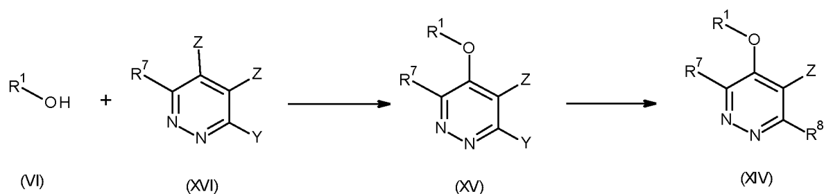
Scheme 10
