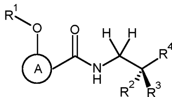
(I-1)
