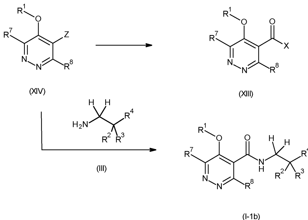
Scheme 9
