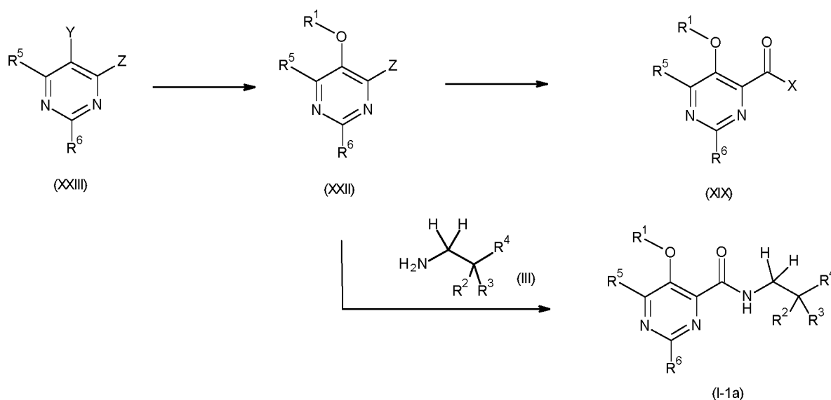
Scheme 15
