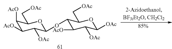
Scheme 10 Synthesis of a Lactose-Derived Acceptor
