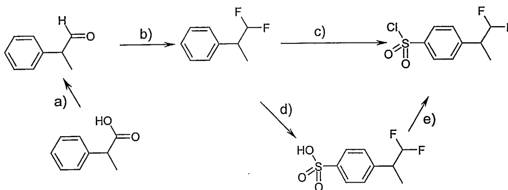
Scheme 7:
