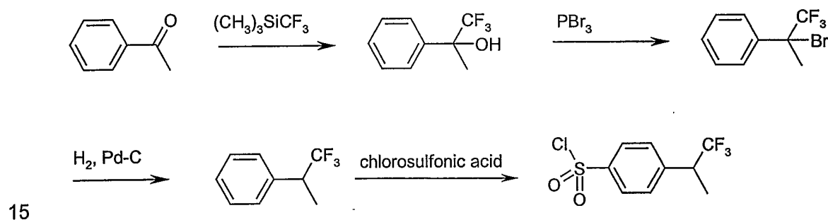
Scheme 9:
