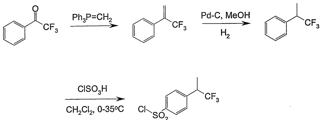
Scheme 8:
