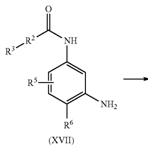
Scheme H: Preparation of compounds of the formula (Ic) from aniline derivatives of formula (XVII)
