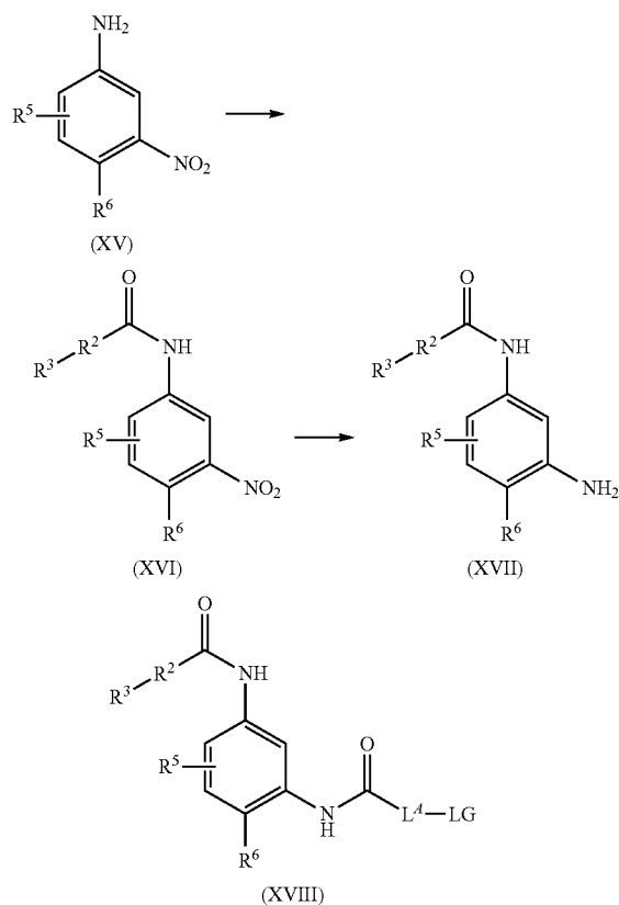
Scheme F: Preparation of compounds of the formula (Ib) from meta-nitroaniline derivatives of formula (XV)
