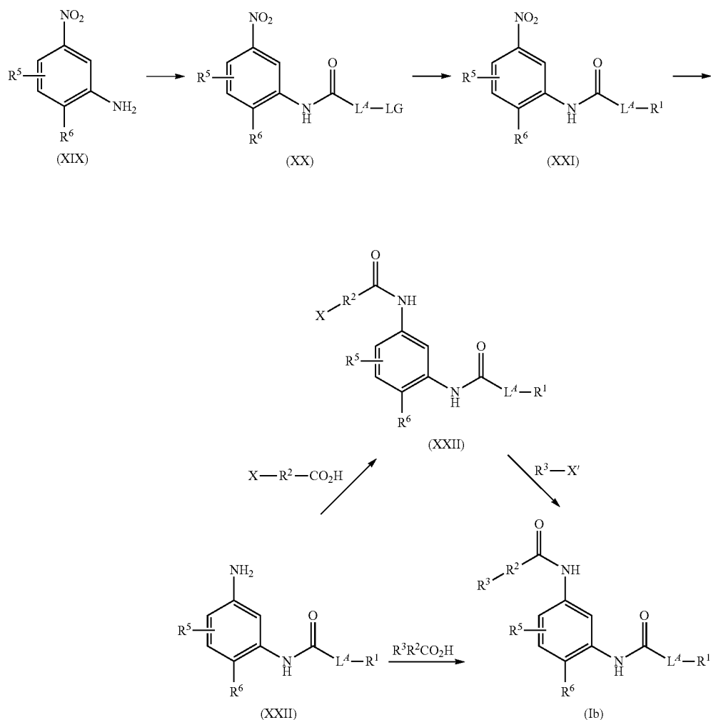
Scheme G: Preparation of compounds of the formula (Ib) from meta-nitroaniline derivatives of formula (XIX)
