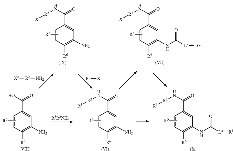
Scheme C: Preparation of compounds of the formula (Ia) from meta-aminobenzoic acid derivatives of formula (VIII)
