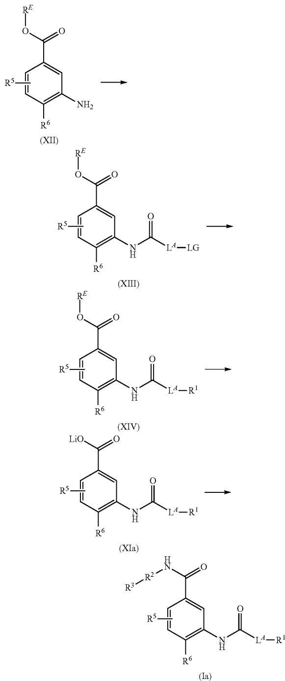
Scheme E: Preparation of compounds of the formula (Ia) from meta-aminobenzoic acid esters of formula (XII)
