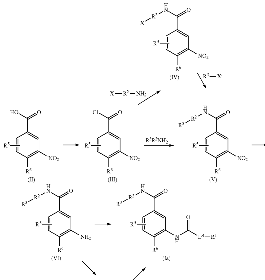
Scheme B: Preparation of compounds of the formula (Ia) from meta-nitrobenzoic acid derivatives of formula (II)
