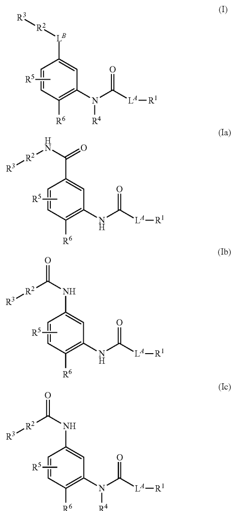
Scheme A: Formulae (I), (Ia), (Ib), and (Ic).
