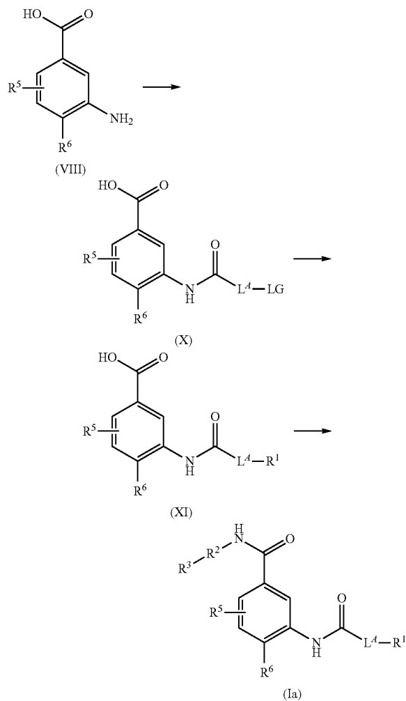
Scheme D: Alternative preparation of compounds of the formula (Ia) from meta-aminobenzoic acid derivatives of formula (VIII)
