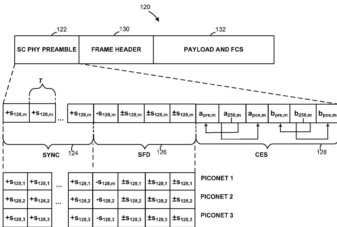
FIG. 3 (PRIOR ART)
