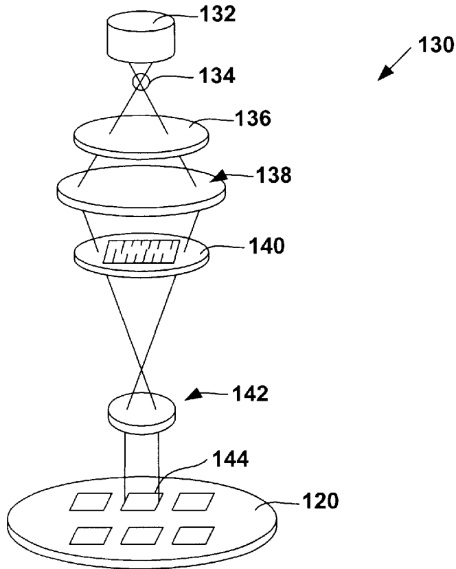
Fig. 2d Prior Art
