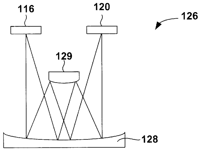
Fig. 2c Prior Art
