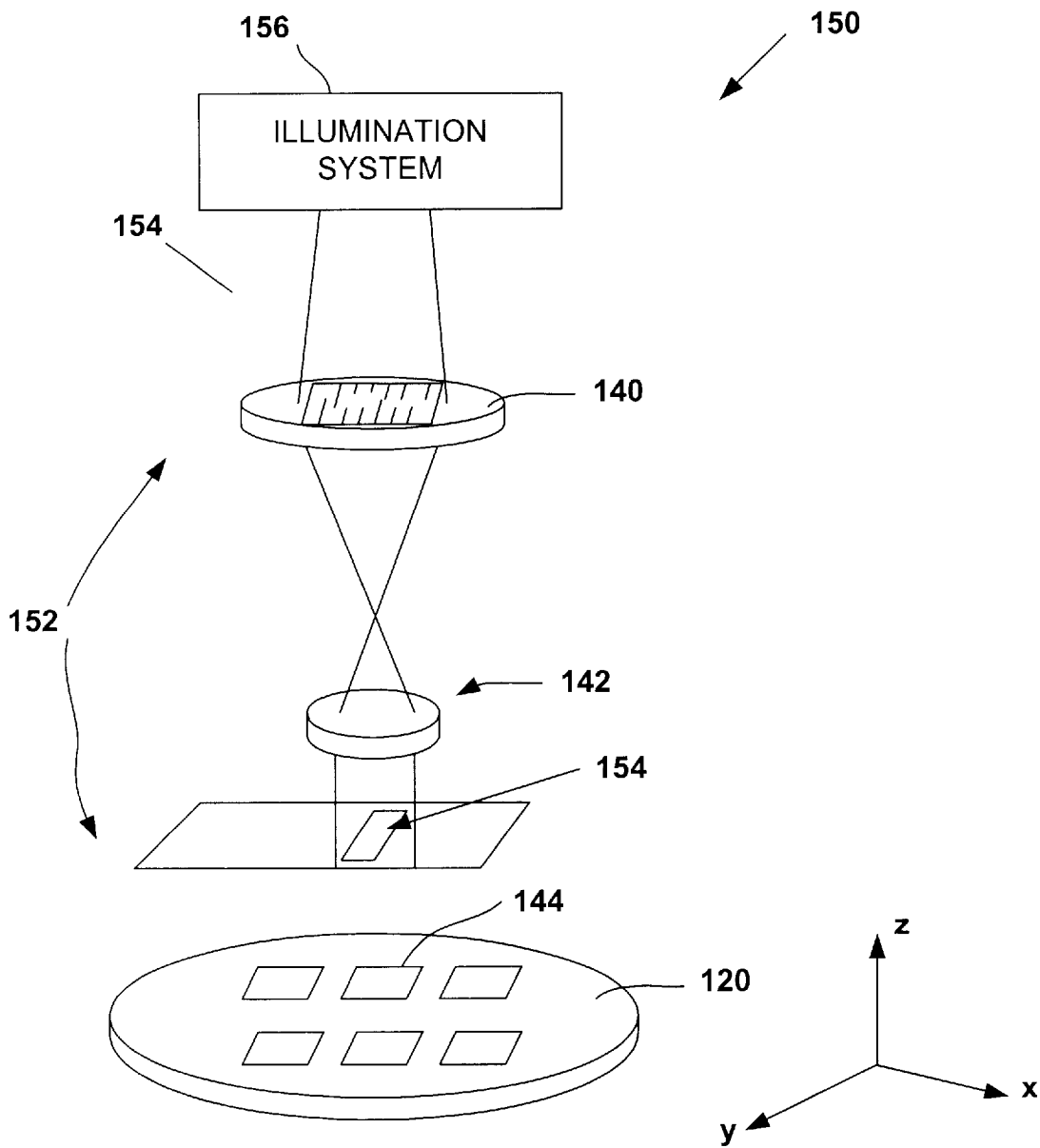
Fig. 3 Prior Art
