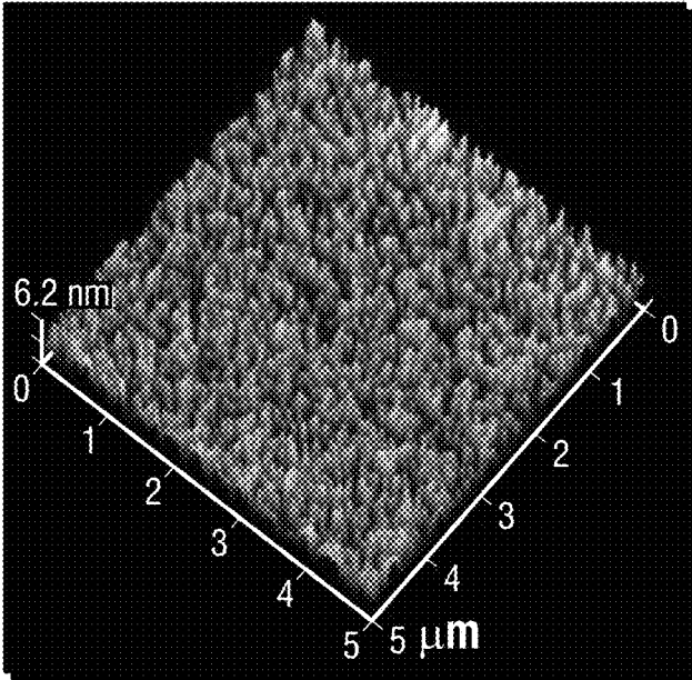
Arg-PEI/siRNA
