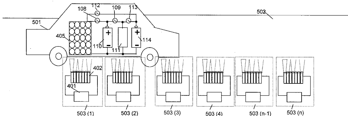
Laser beam coupled Wireless charger for vehicles embedded on a road
