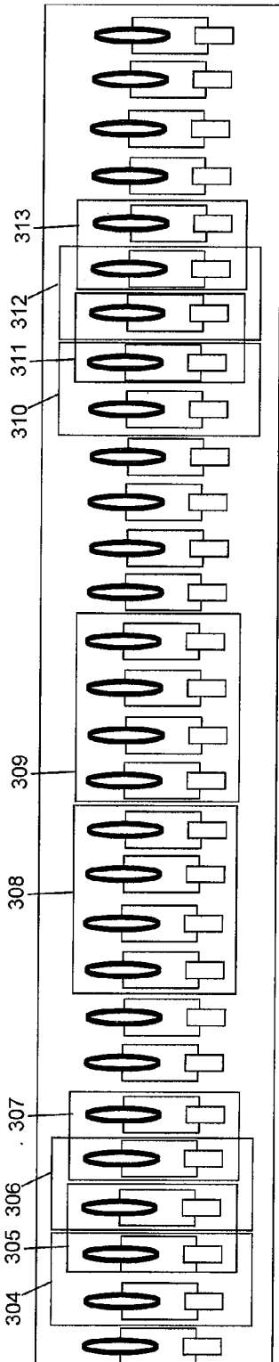
Fig. 3B Continuous Wireless Chargers on a road
