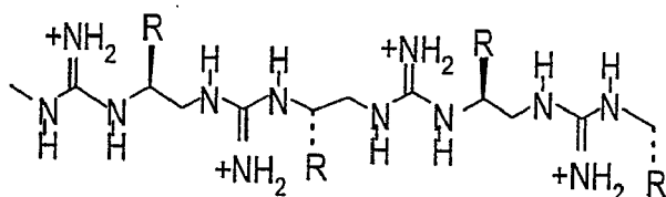
Polyguanidiniums
