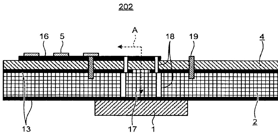
FIG.7 BACKGROUND ART
