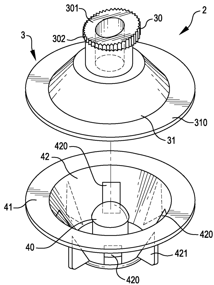
FIG. 2 PRIOR ART
