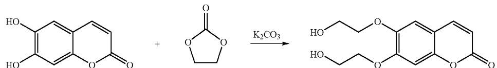
Reaction Scheme (II)
