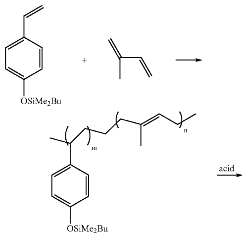
Reaction Scheme (V)
