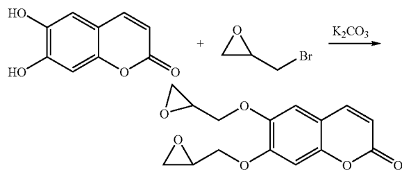
Reaction Scheme (VI)
