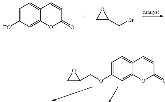
Reaction Scheme (IV)
