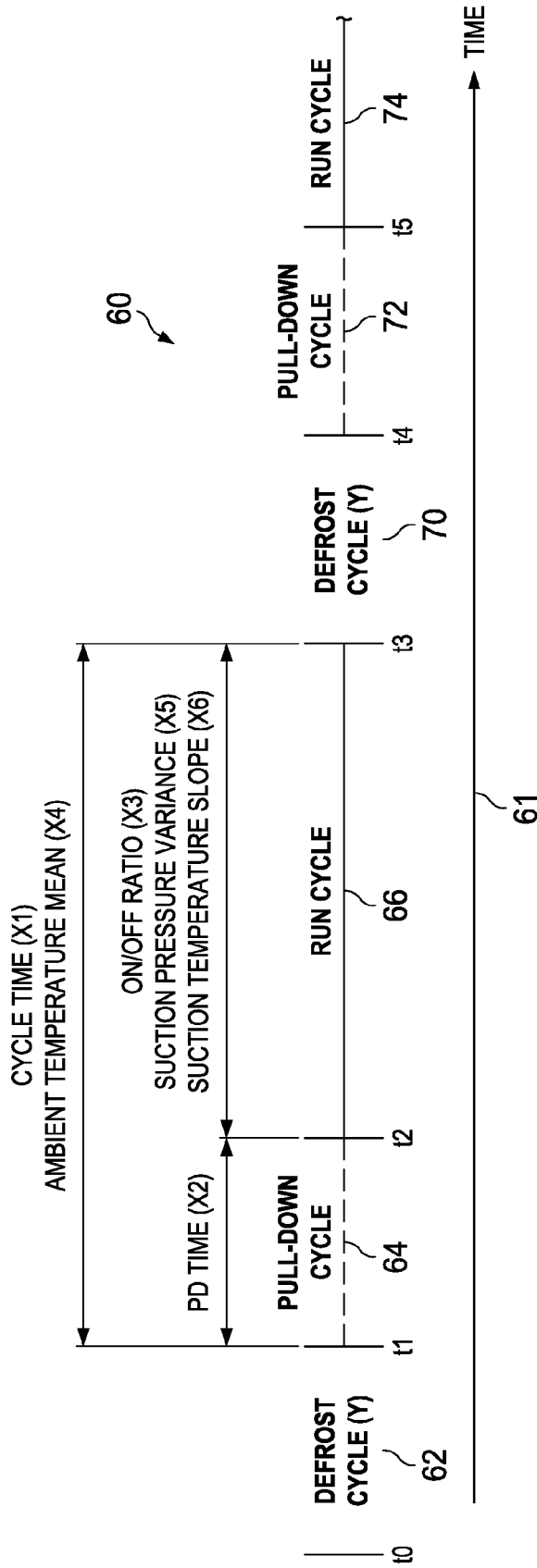
FIG. 2 (PRIOR ART)
