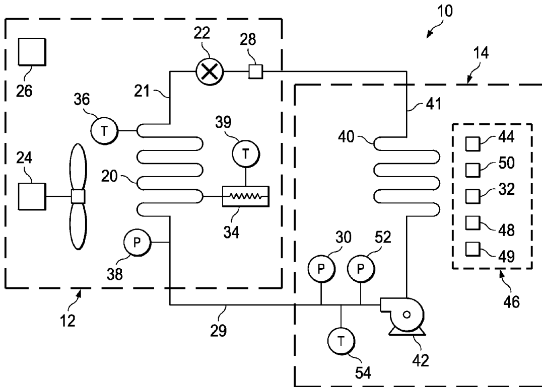
FIG. 1 (PRIOR ART)
