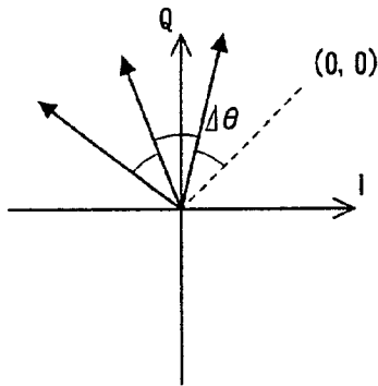
PHASE ERROR
