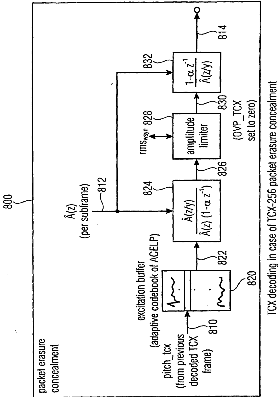
Block diagram of the TCX decoder FIG 8
