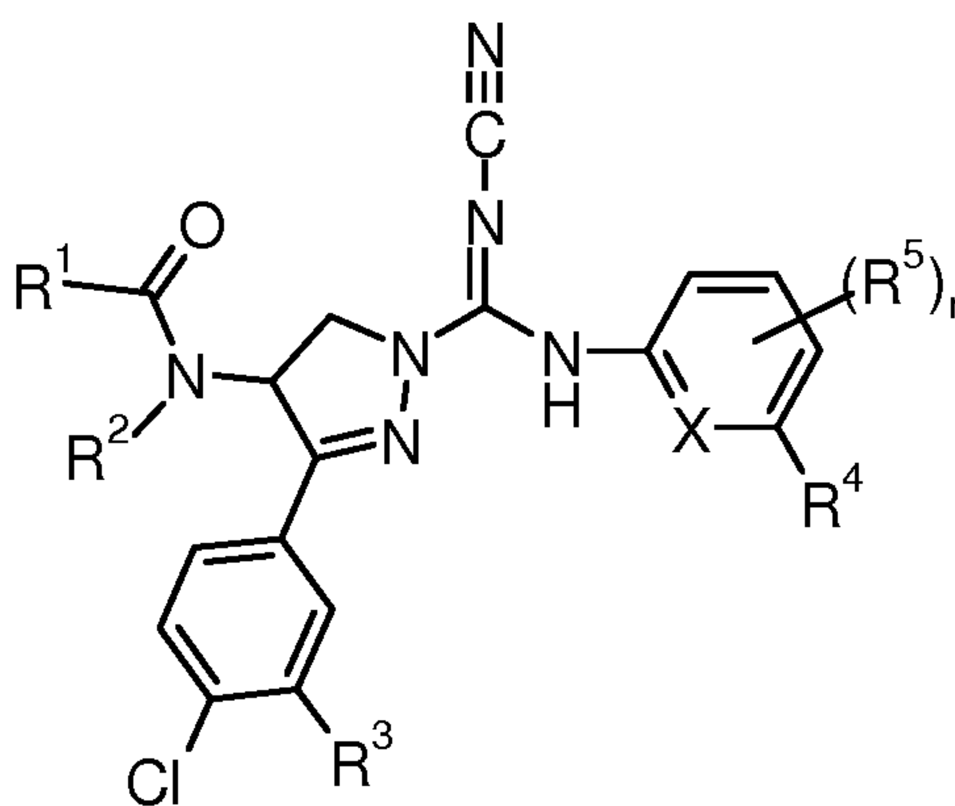
(I)
