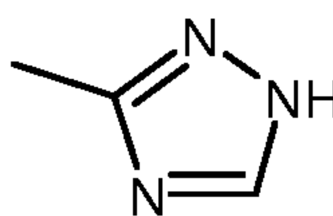
2H-tautomer
