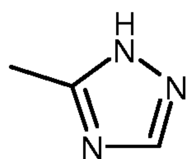
1H-tautomer
