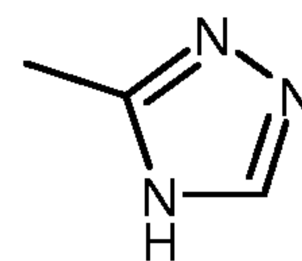
4H-tautomer
