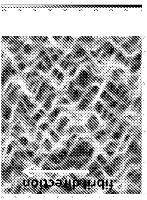
FIG. 6A. Align-braided
