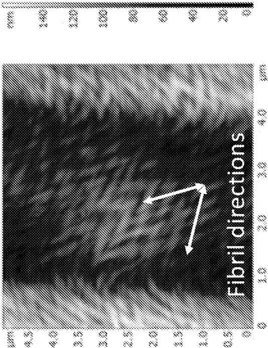
FIG 6C. Basket-Weave
