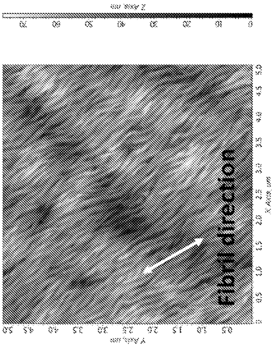
FIG. 6D. Cornea-like
