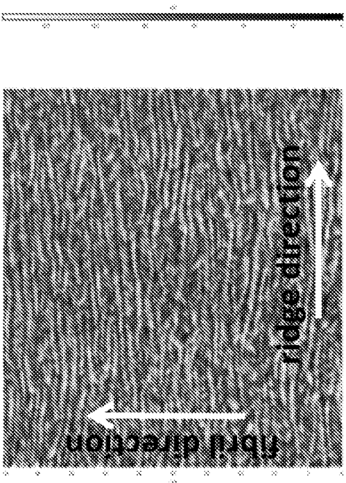
FIG. 6B. Tendon-like
