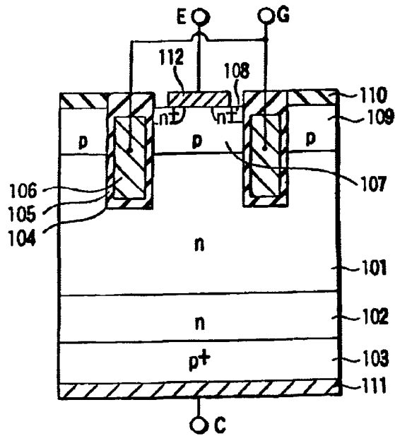
FIG. 25 PRIOR ART
