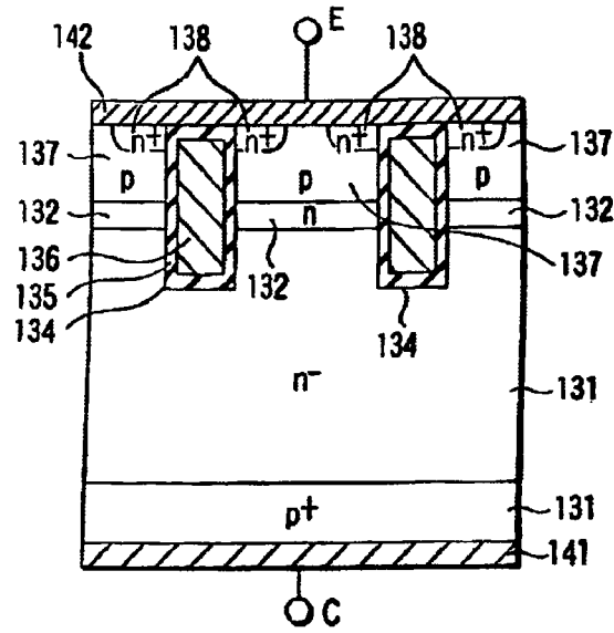
FIG. 26 PRIOR ART
