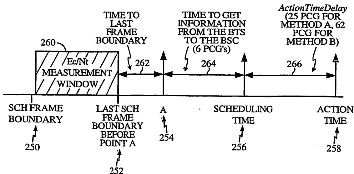
SCHEDULING DELAY TIMING FIG. 3
