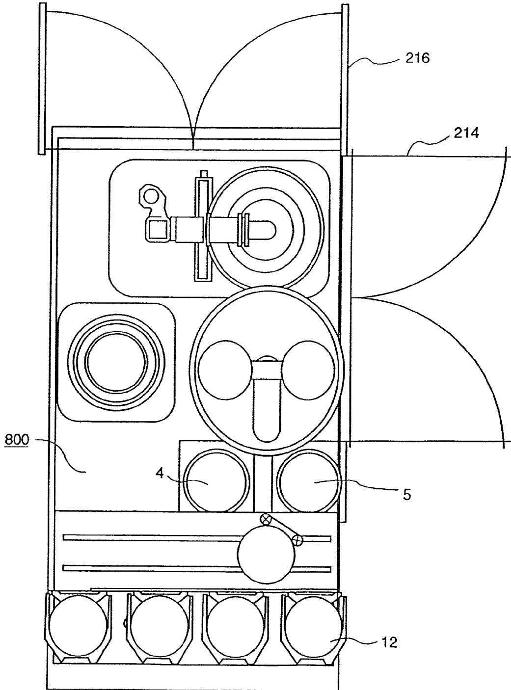
FIG. 9 PRIOR ART
