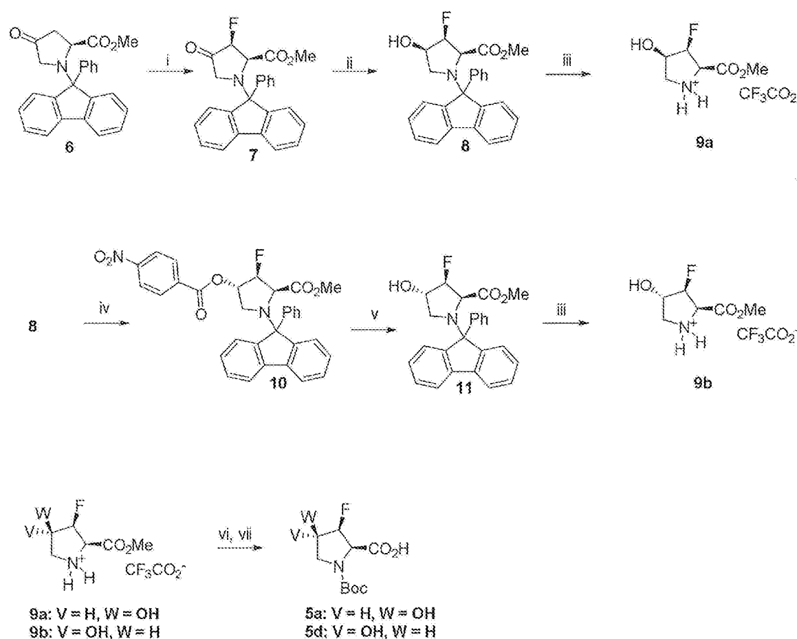
Scheme 2
