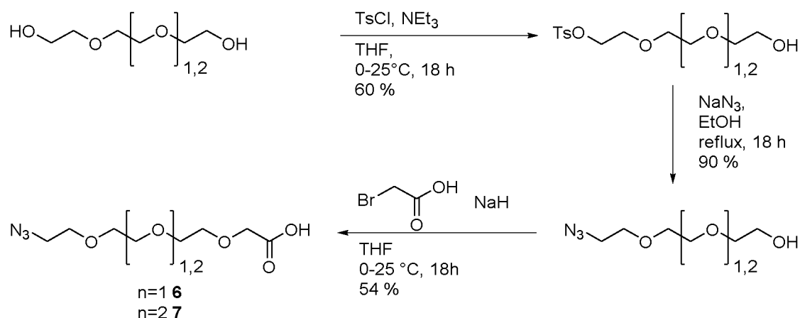
Scheme 6
