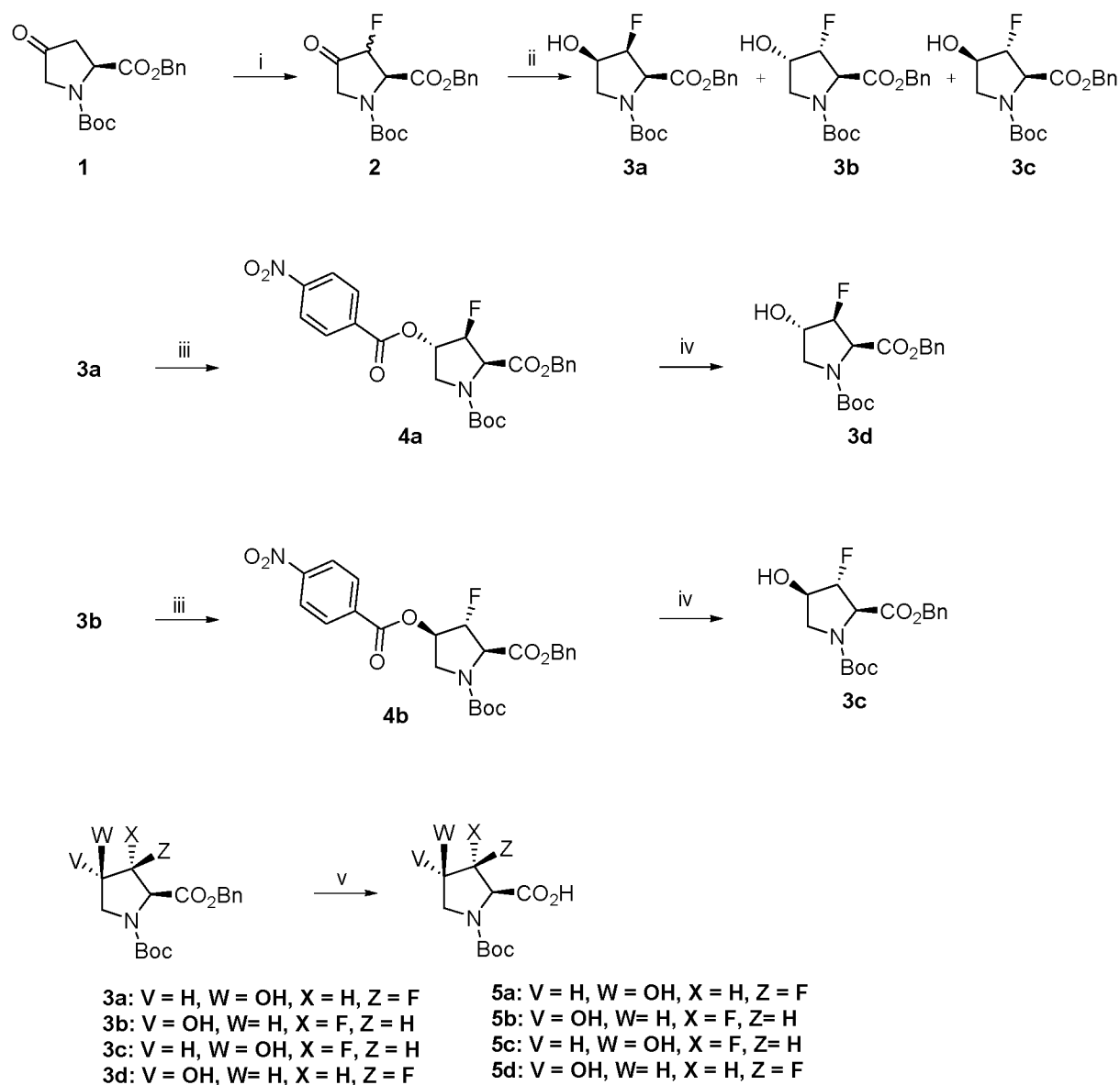
Scheme 1
