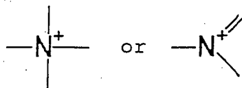
ammonium salts
