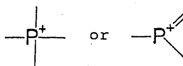
phosphonium salts
