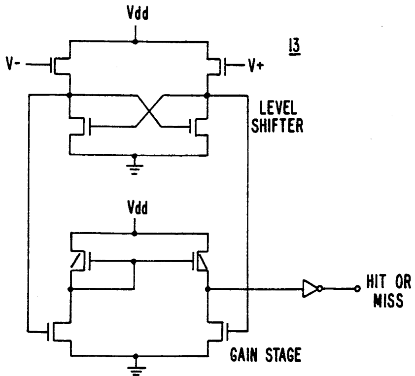
FIG. 6. PRIOR ART
