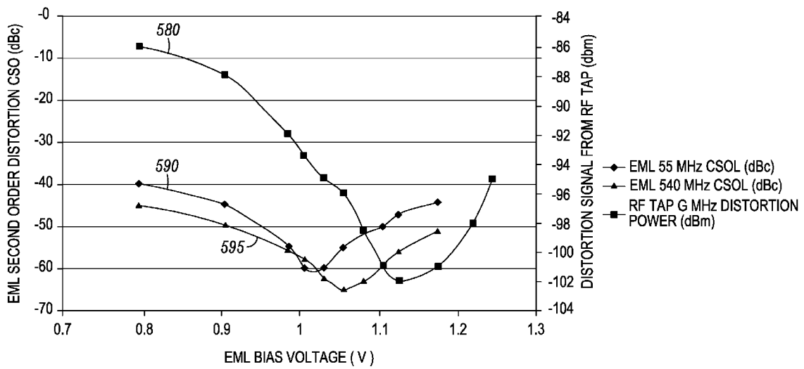
CORRELATION BETWEEN EML SECOND ORDER DISTORTION AND RF DISTORTION PRODUCT
