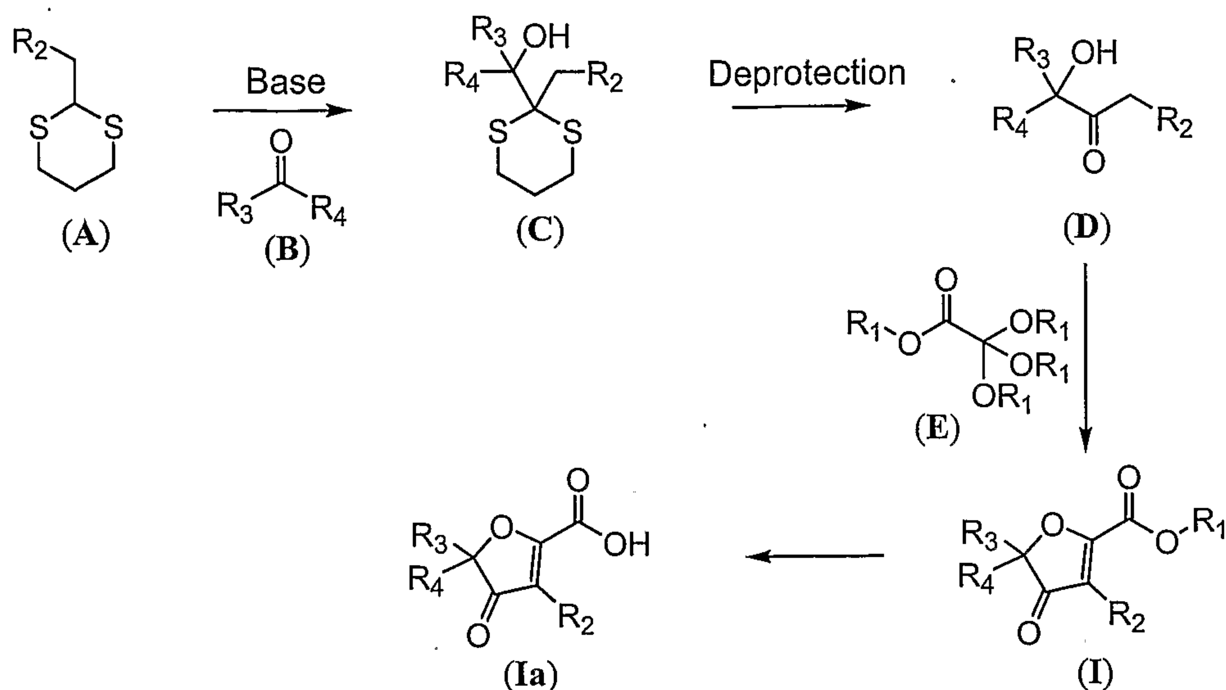
Reaction Scheme (1)
