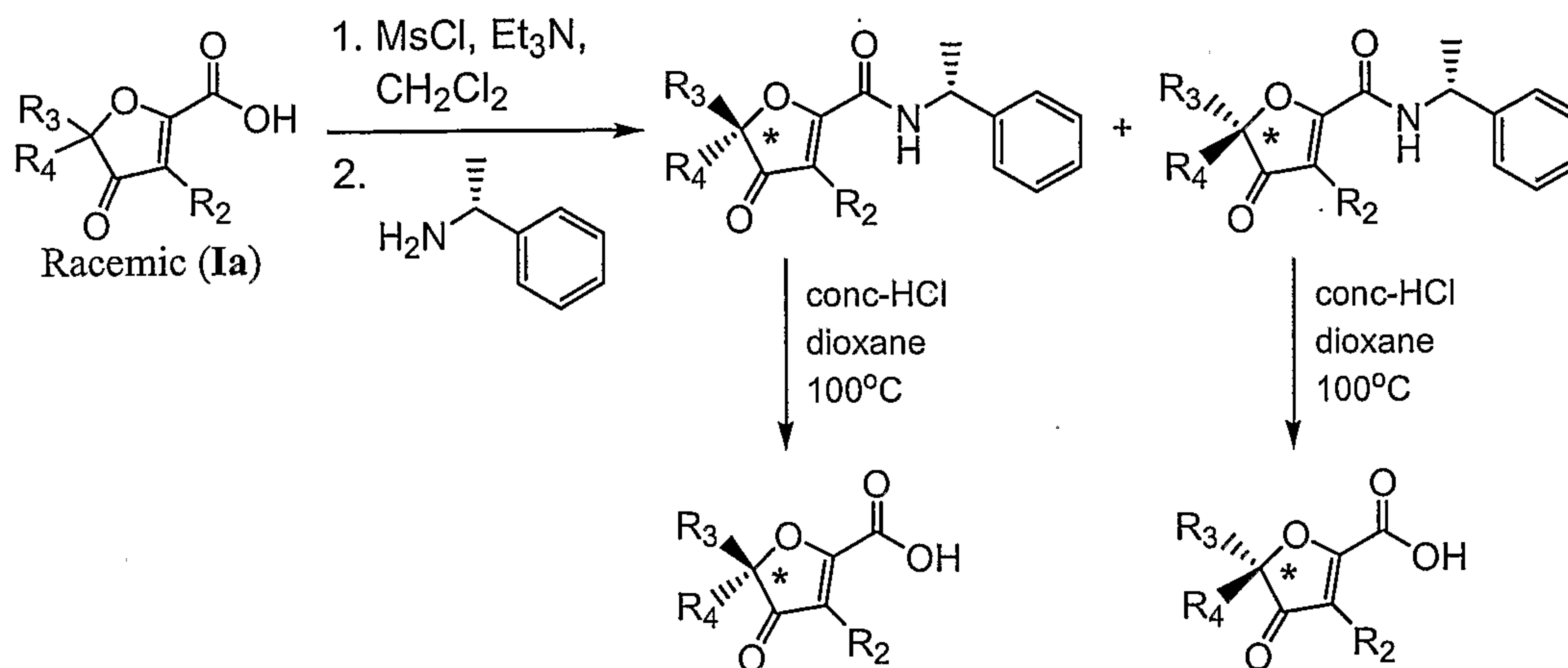
Reaction Scheme (4)
