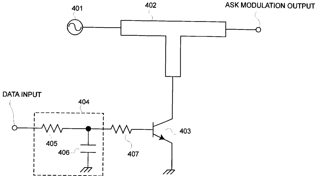
FIG.19 PRIOR ART
