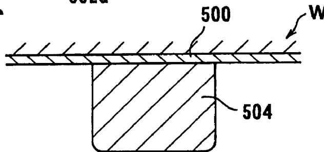
FIG. 29C PRIOR ART
