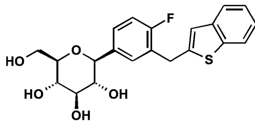
(9) Ertugliflozin, represented by formula (9):
