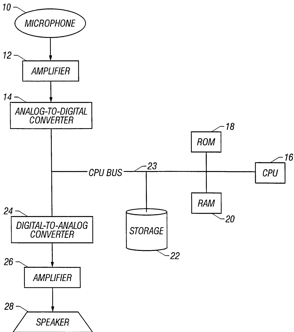
FIG. 1 (Prior Art)
