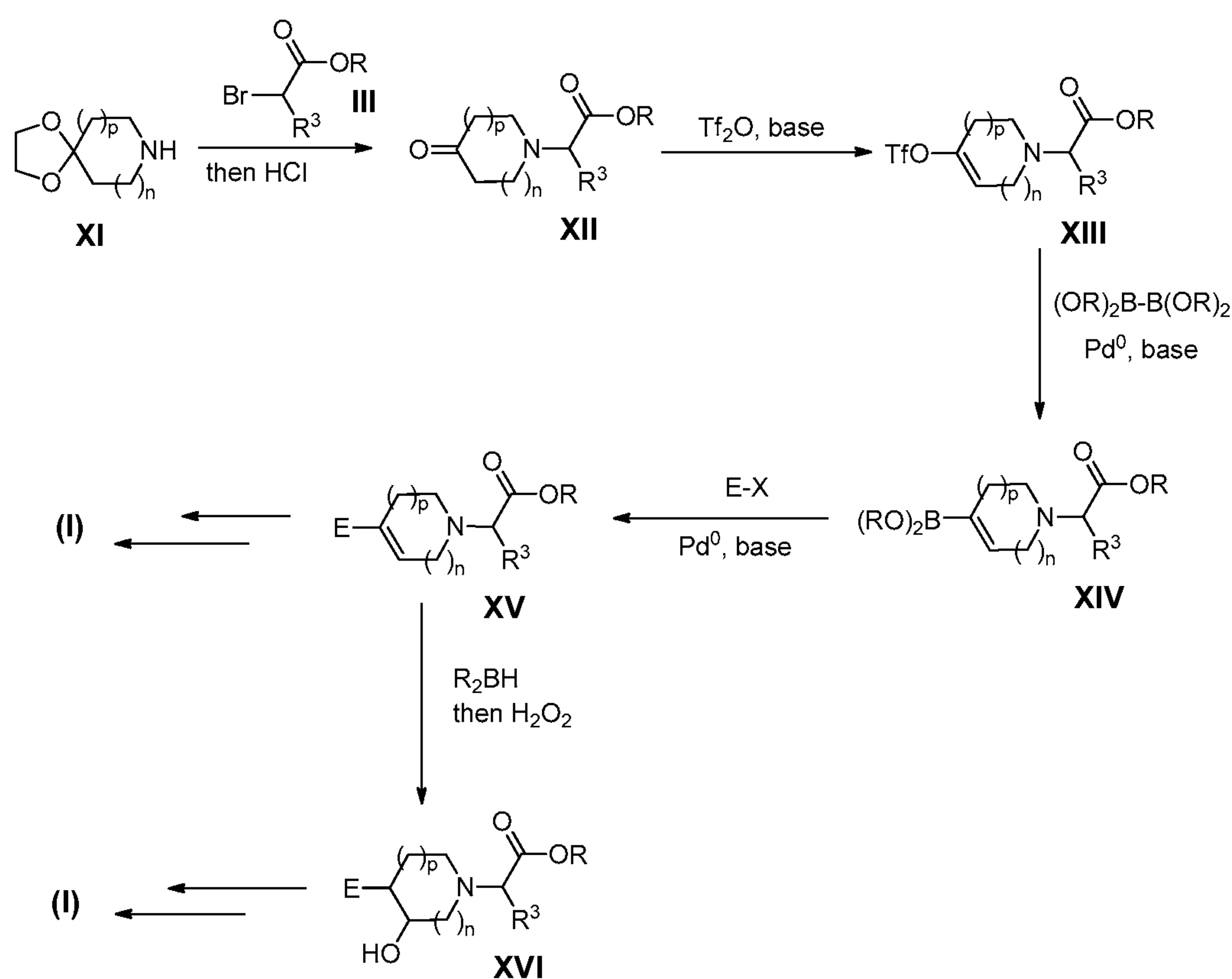
Scheme 3
