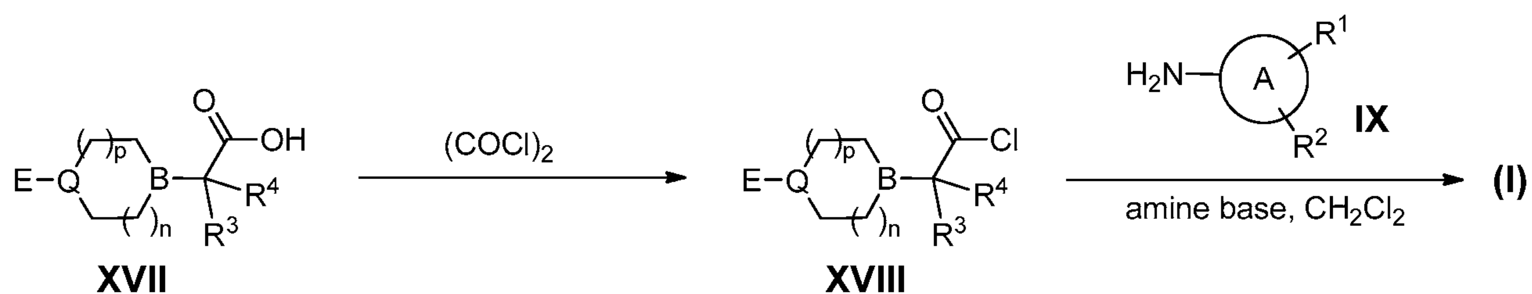
Scheme 4
