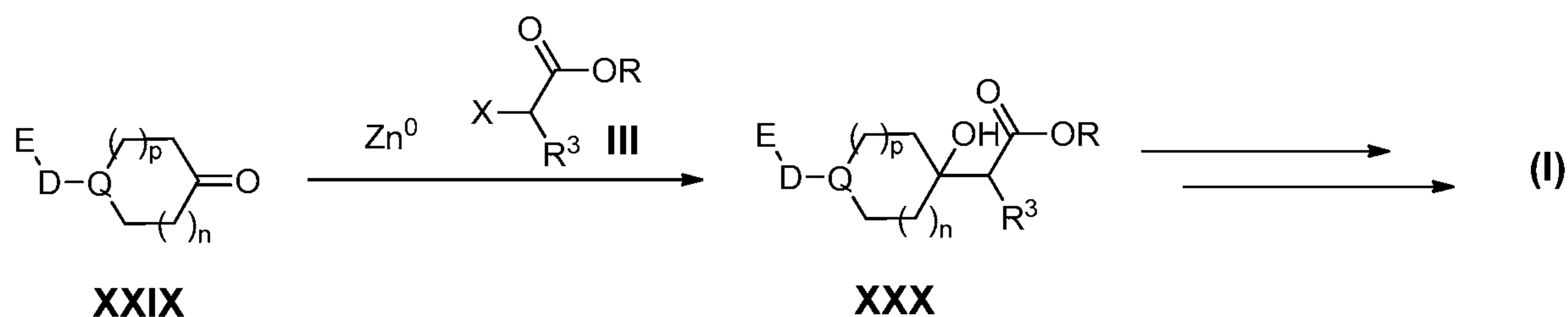
Scheme 8
