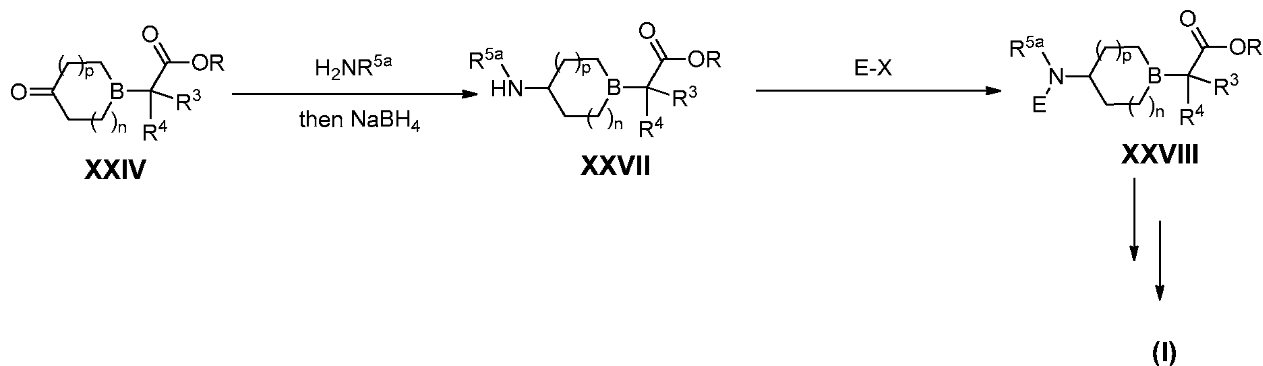
Scheme 7
