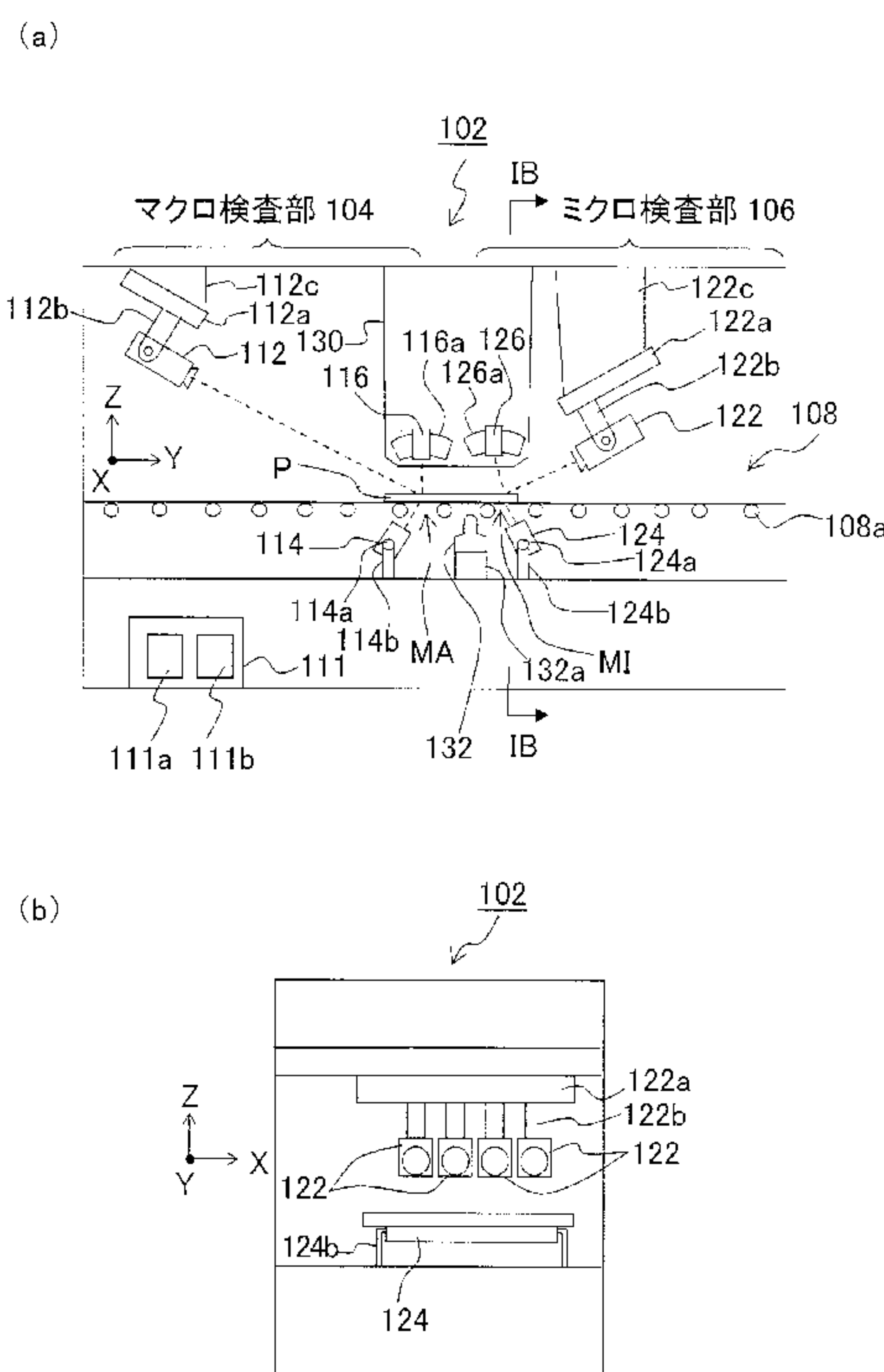
FIG. 2: 104 Macro inspection unit 106 Micro inspection unit
