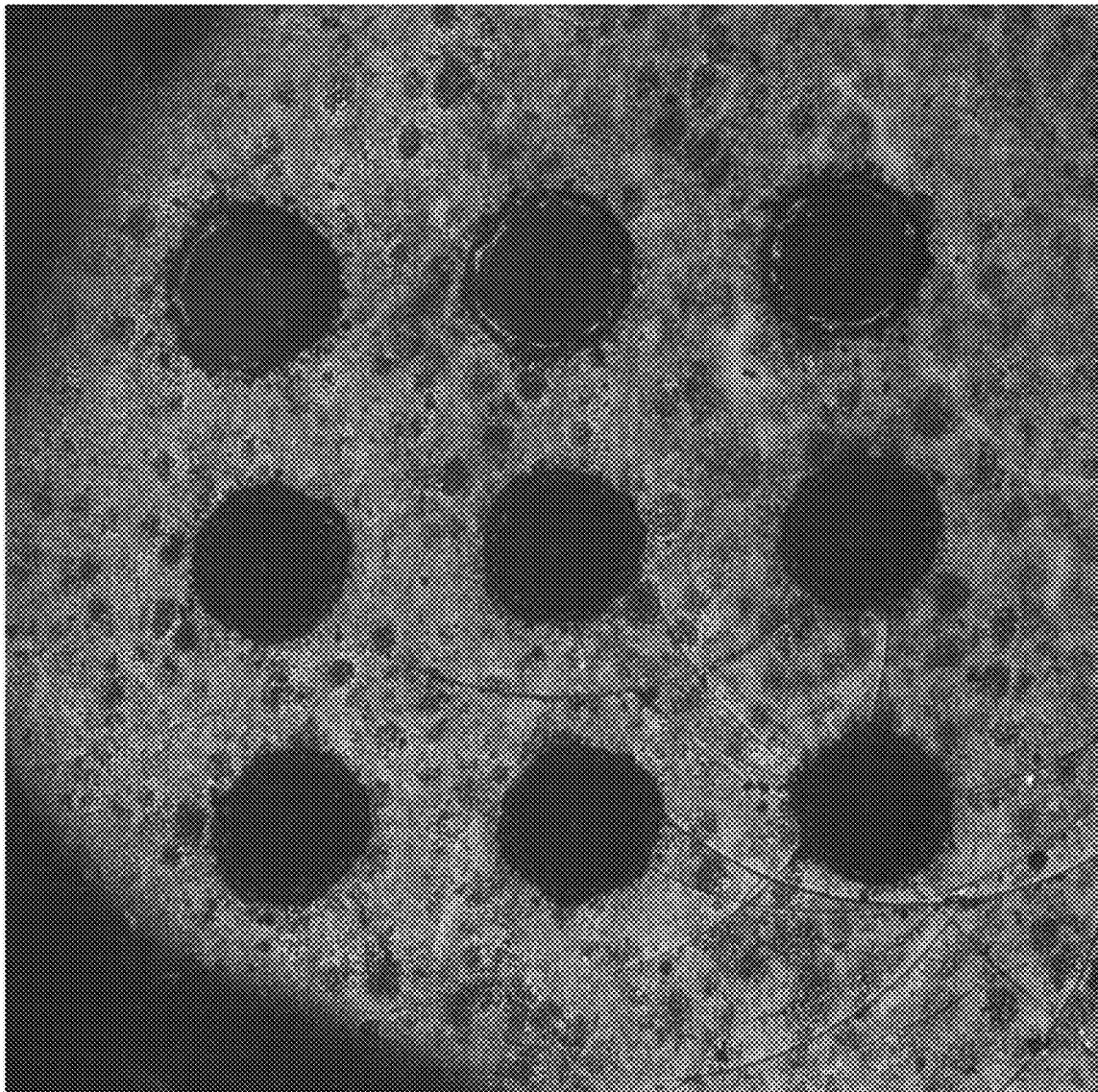
40uS ON-Time, 20 Pulses per Crater
