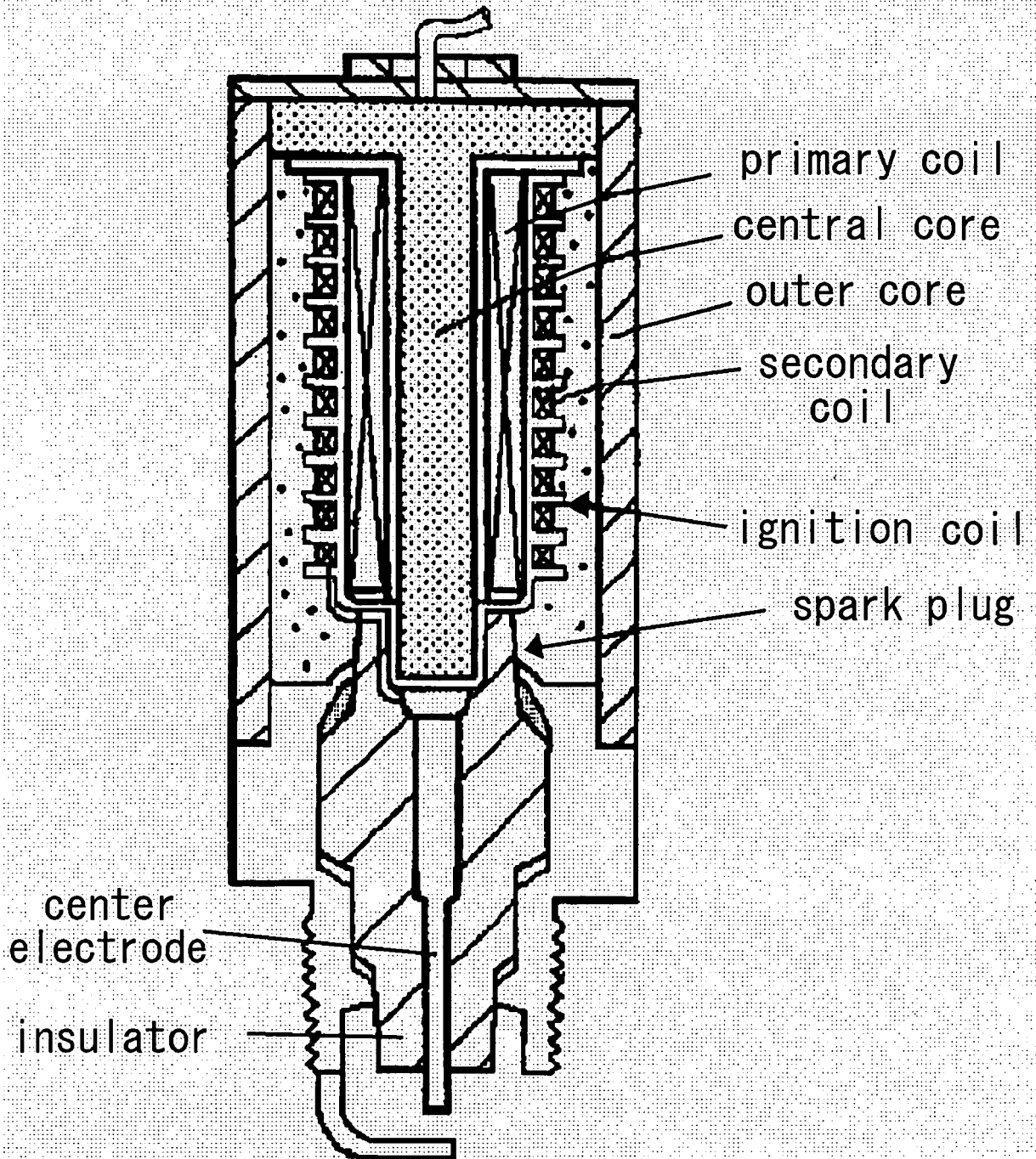
Fig.5 Prior Art
