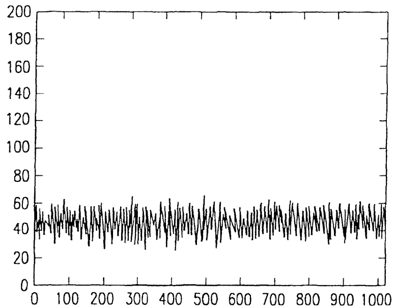
FIG. 10 APERIODIC CROSS- CORRELATION OF THE COMMA FREE CODES
