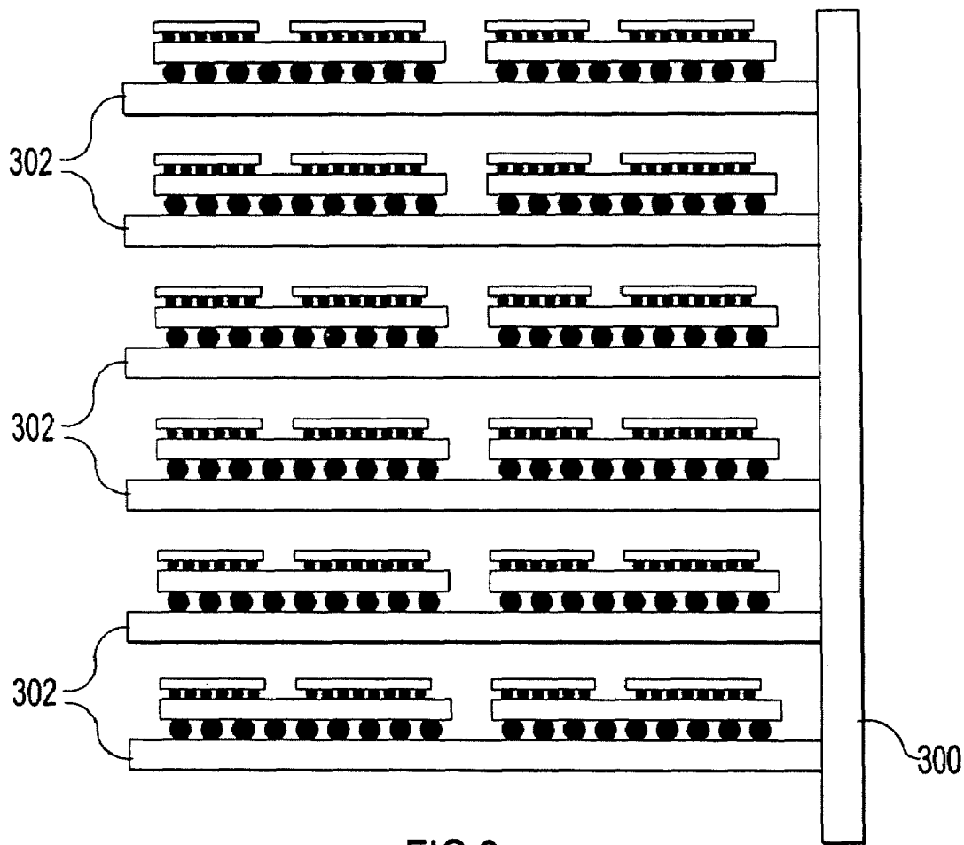
FIG. 3 (PRIOR ART)
