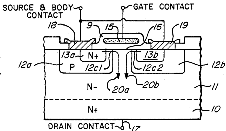
FIG. 1 (PRIOR ART)
