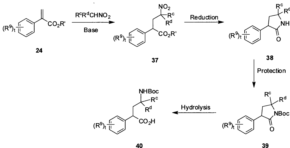
Scheme D
