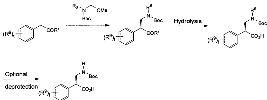
Scheme J
