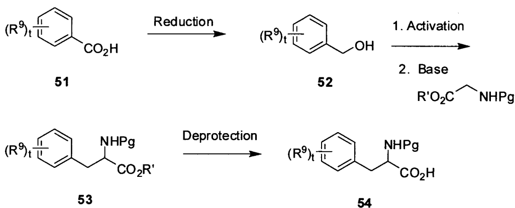
Scheme G
