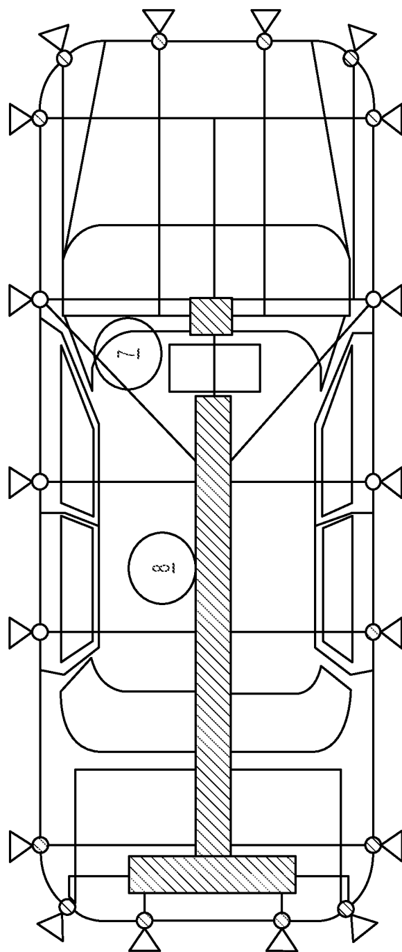
SYSTEM ARCHITECTURE (MULTIPLE SENSORS VIA ETHERNET) (360° SENSING)
