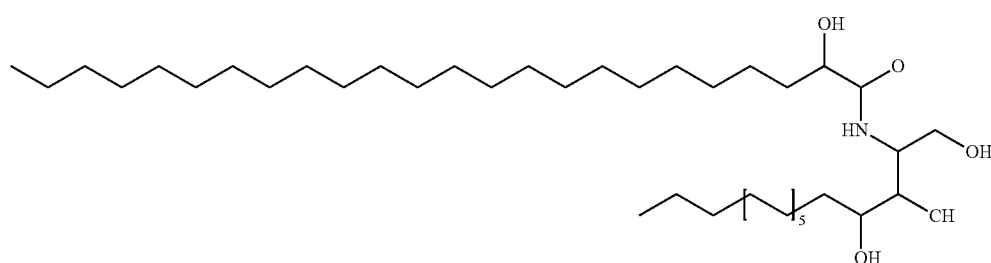
Ceramide 6 (Type II)
